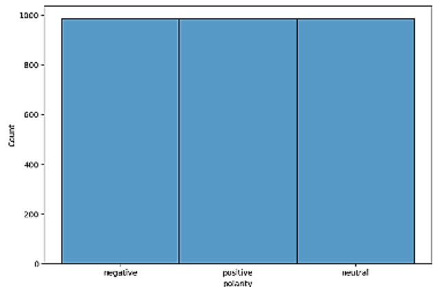
Figure 16. After SMOTE, Arifin Setiono
