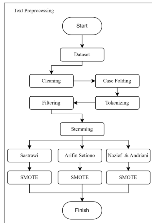
Figure 3. Workflow of Text Preprocessing
